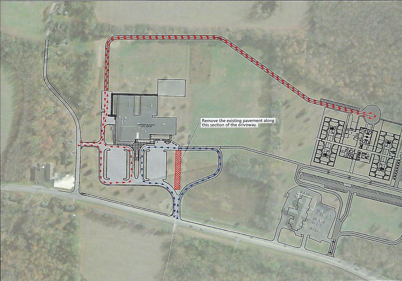
Figure 12A - Option 1 Recommended Improvements Smithville Elementary School • Smithville, TN • Scale: 1" = 200' Prepared by T-Square Engineering, Inc. 701 West Main Street • Franklin, TN 37064 • www.T2-Eng.com
